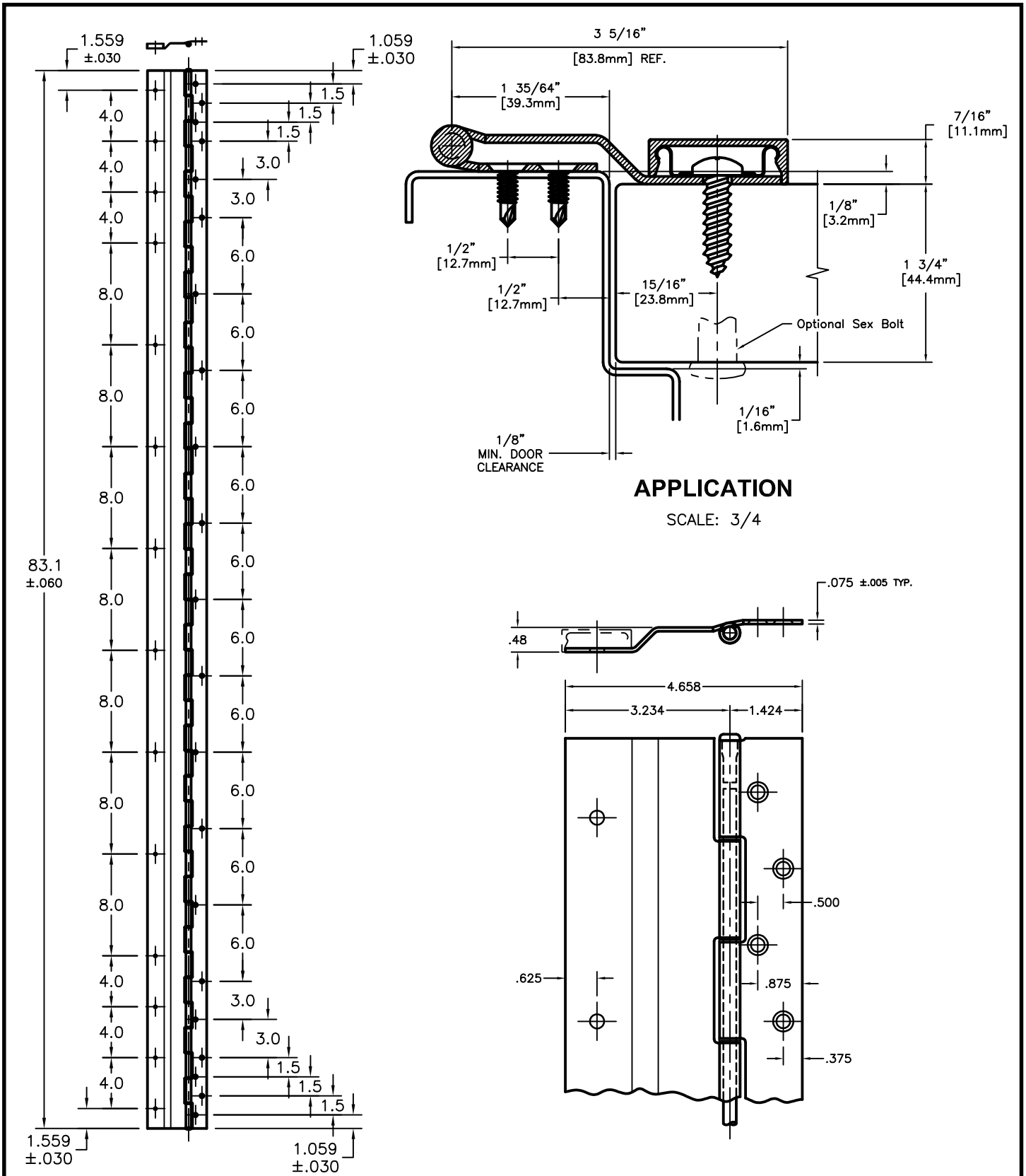
HOLE PATTERN DETAIL SCALE: 3/8
